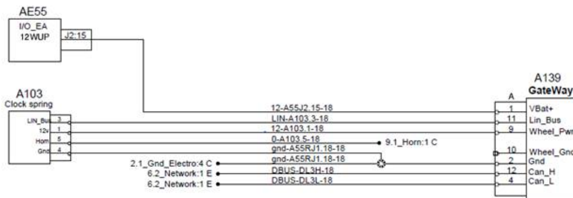
Wiring diagram with EFD (before modification)
