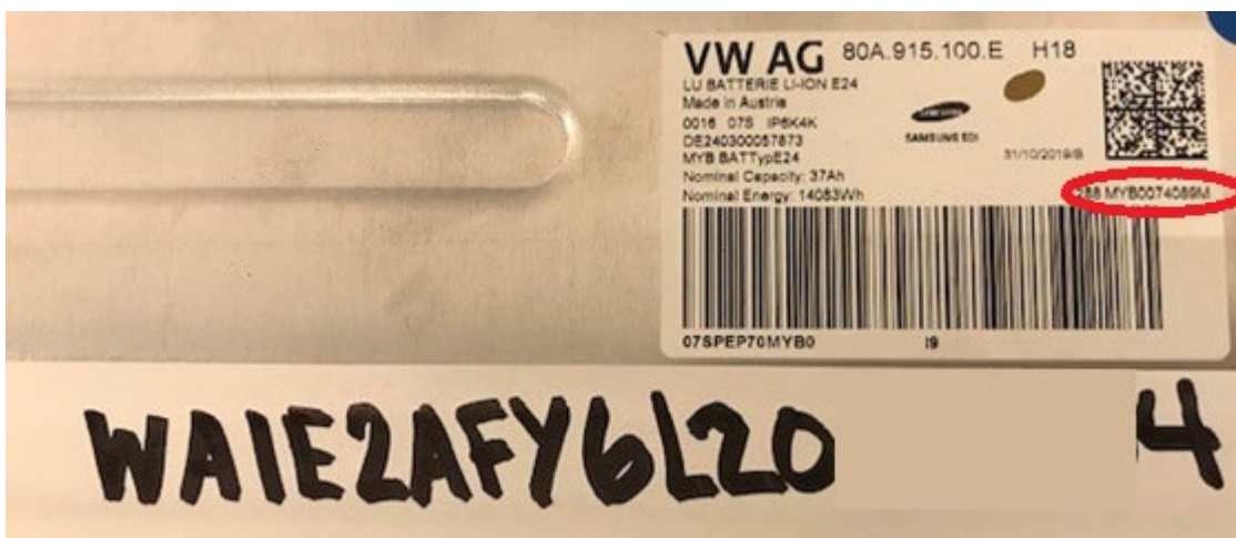
Figure 2. Cell Module identification from an Audi Q5 PHEV.
