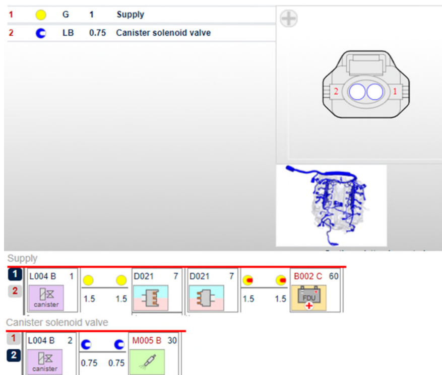
2 way purge valve wiring diagram.
