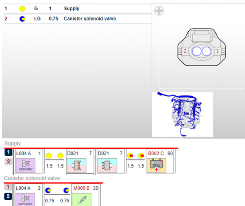
3 way purge valve wiring diagram.
