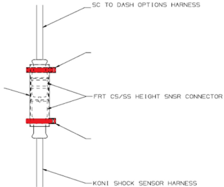
Figure 8: Connector with Shrink Tube & Tyraps.
