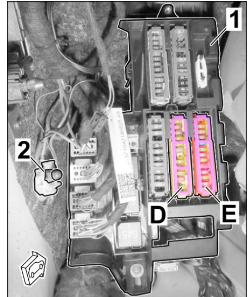
Figure 5 (LHD vehicle)
