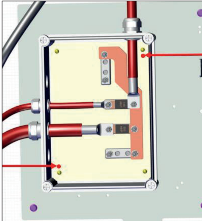
Figure 8: Position of holes
