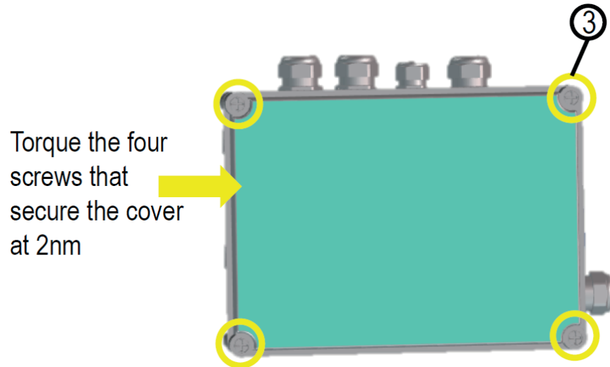
Figure 12: Torque for Cover Screws
