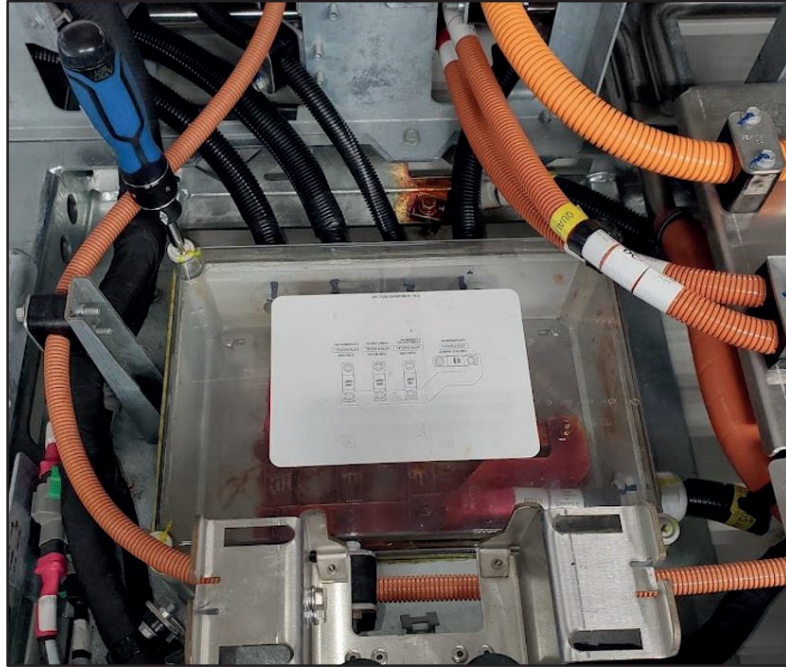
Figure 3: Loosen cover screws with #3 Philipps screwdriver
