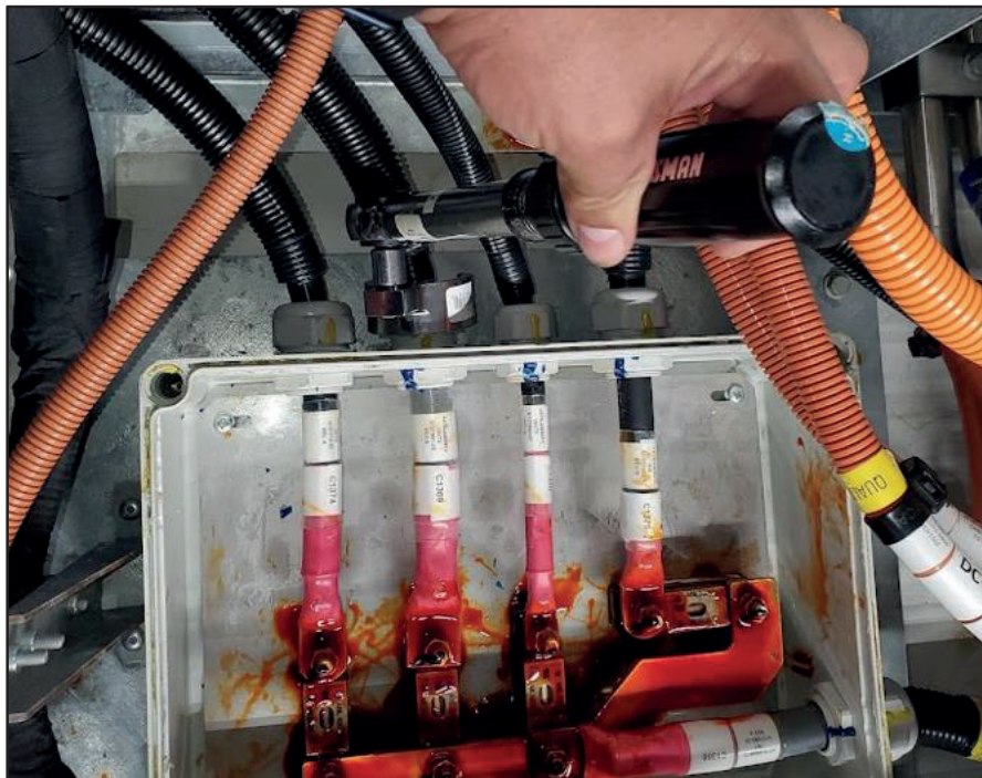
Figure 6: Loosen the cable gland dome nuts
