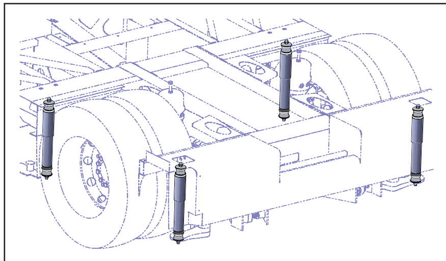
Figure 4 - Location of Rear Shock Absorbers
