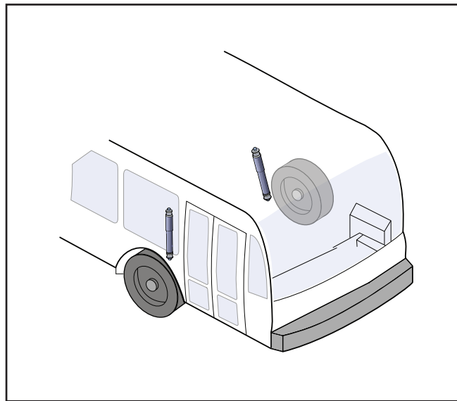
Figure 3 - Location of Front Shock Absorbers
