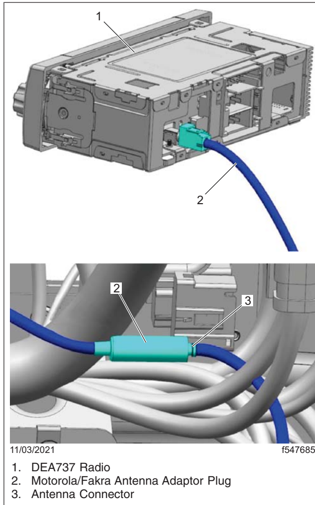
Fig. 1, Installing a Replacement CAN-Connected Radio and Antenna Adaptor
