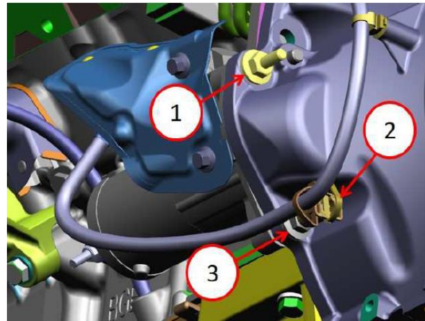
Figure 1 – Starter Mounting Studs
