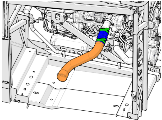
FIGURE 140: CONNECTION AT THE TURBO OUTLET ELBOW
