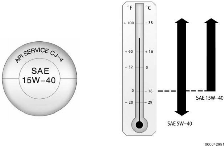
Figure 6 Oil Viscosity Grades and Temperature Ranges
