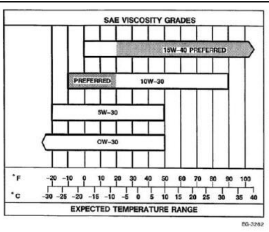
Figure 22 SAE Viscosity Grades and Temperature Ranges
