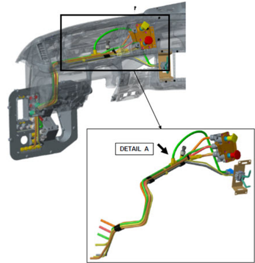
DETAIL A
