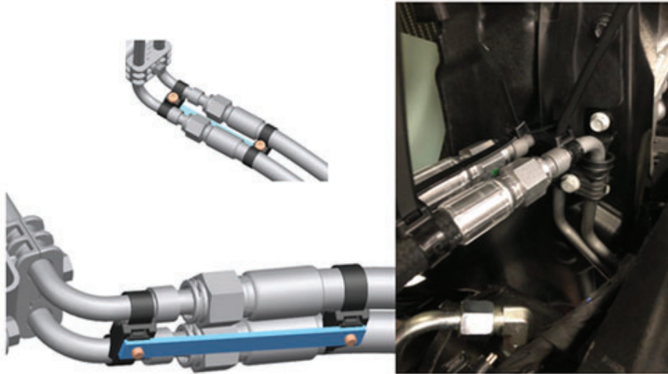
Retainer assembly
