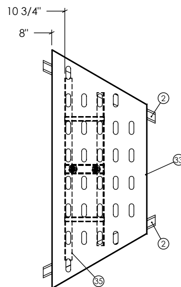
DETAIL F SCALE 1 : 20
