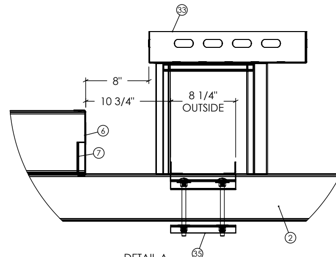
DETAIL A SCALE 1 : 12
