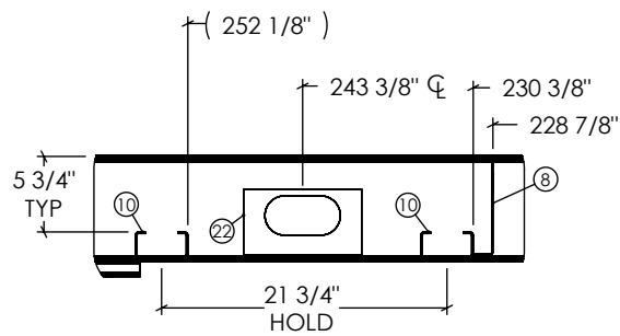
DETAIL C SCALE 1 : 16
