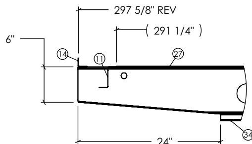
DETAIL E SCALE 1 : 16
