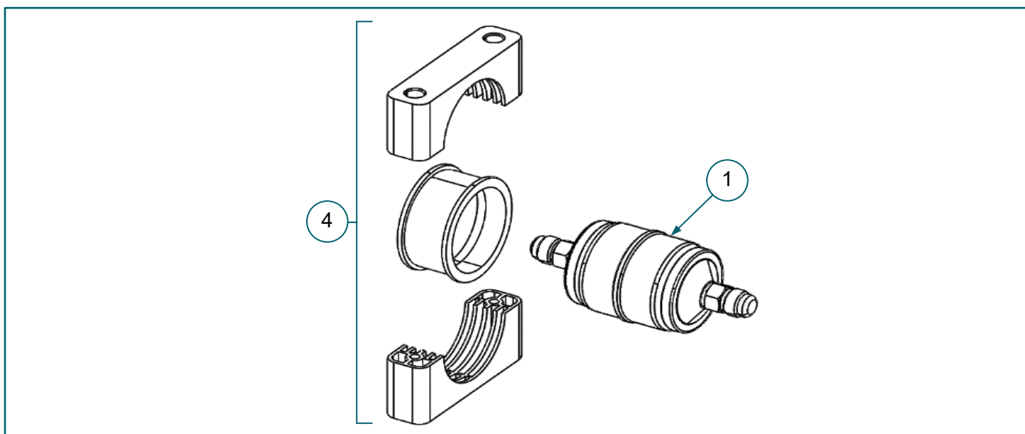
FIGURE 3. Gen 2 HP filter with upgrade Kit, LPG Gen 2 filter mount, p/n 69000573
