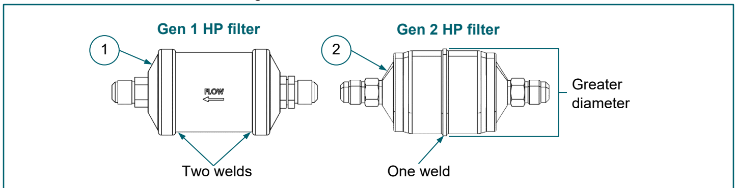
FIGURE 1. HP fuel filter identification
