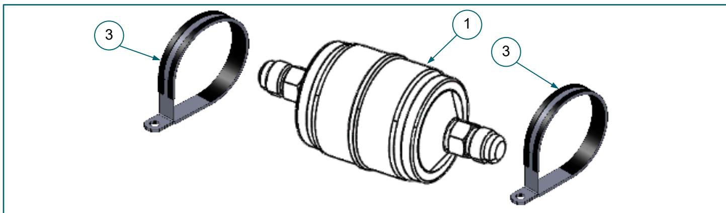
FIGURE 2. HP fuel filter P-clamp mounting
