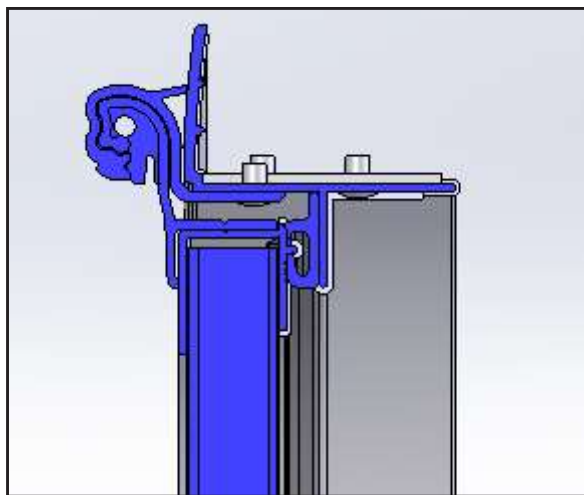
Current inner hinge extrusion with outer extrusion.
