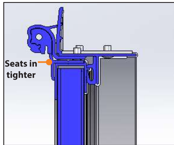
New inner hinge extrusion with outer extrusion.
