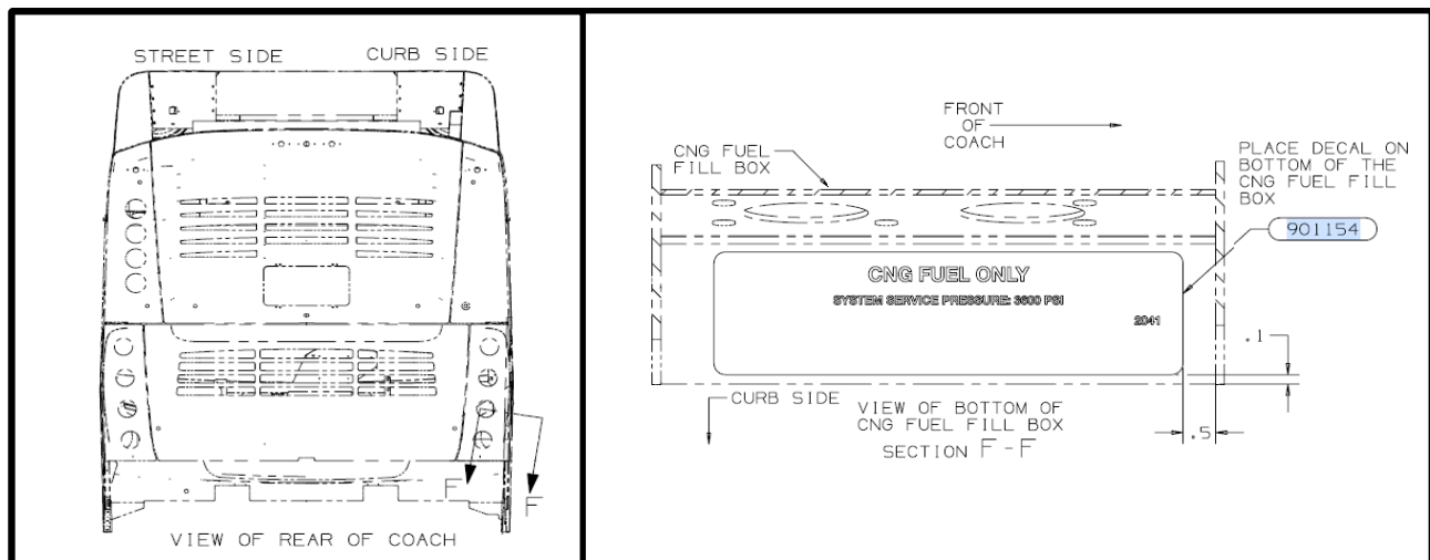
Figure 1: CNG Decal Location Reference.
