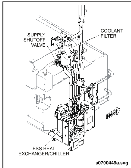
Fig. PM-95: ESS Battery Coolant Filter
