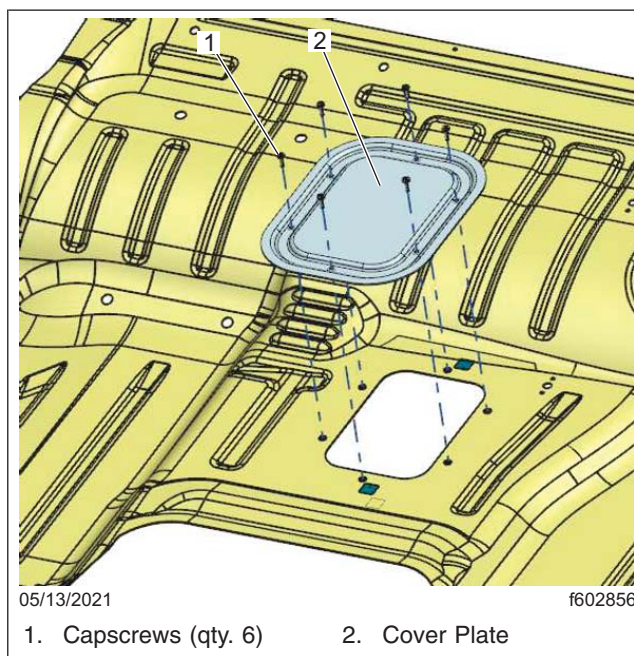
Fig. 1, Installing an Insulated Automatic Transmission Cover Plate
