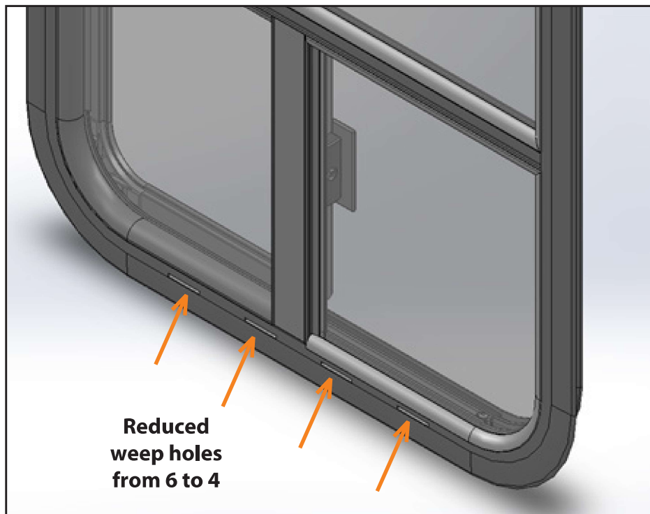
8800BT shown with 4 weep holes for widths larger than 60".
