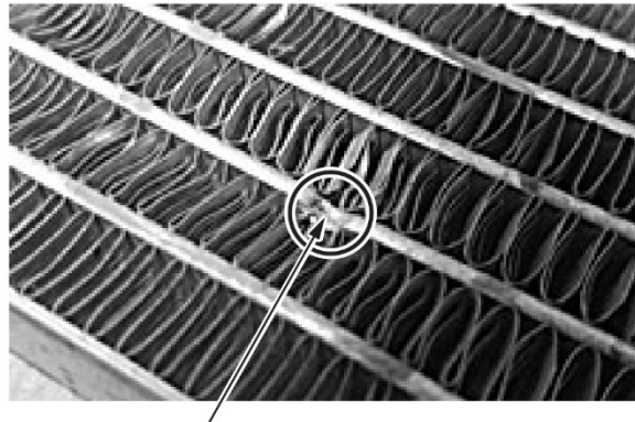
Impact damage on the tube face.
