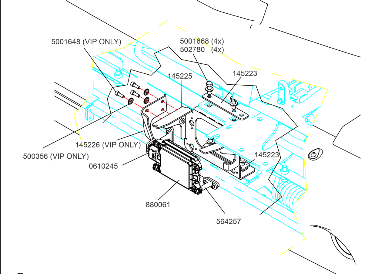
FIGURE 7: FLR21 RADAR INSTALLATION OVERVIEW
