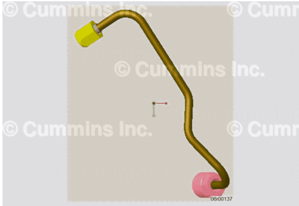
Figure 14, Existing High-Pressure Injector Supply Line, Part Number 4936196 (Injector 6).
