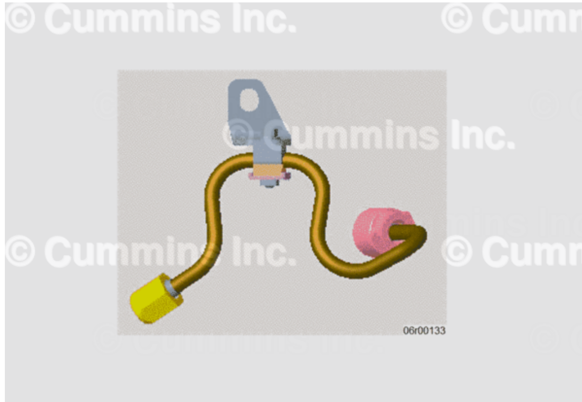
Figure 10, Existing High-Pressure Injector Supply Line, Part Number 4937934 (Injector 4).
