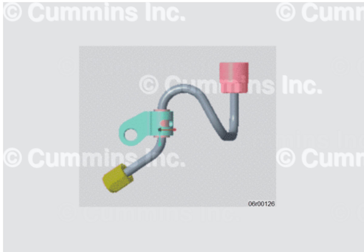
Figure 3, New High-Pressure Injector Supply Line, Part Number 5481953 (Injector 1).
