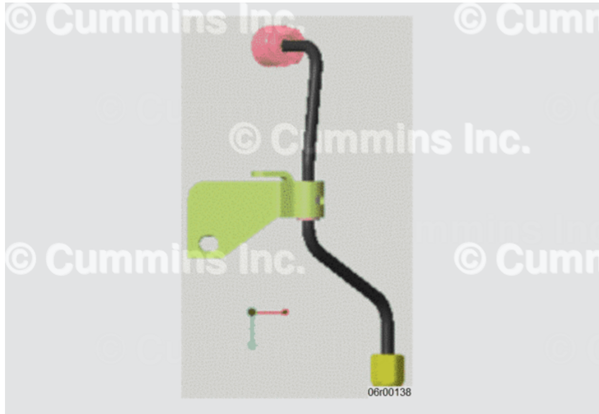
Figure 15, New Fuel Supply Line, Part Number 5525526 (Pump to Rail).
