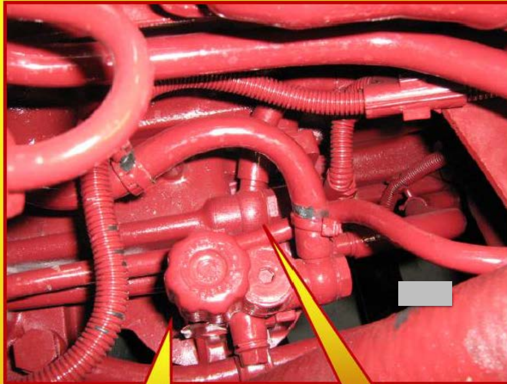
Fuel Filter Base and Hand Priming Pump
