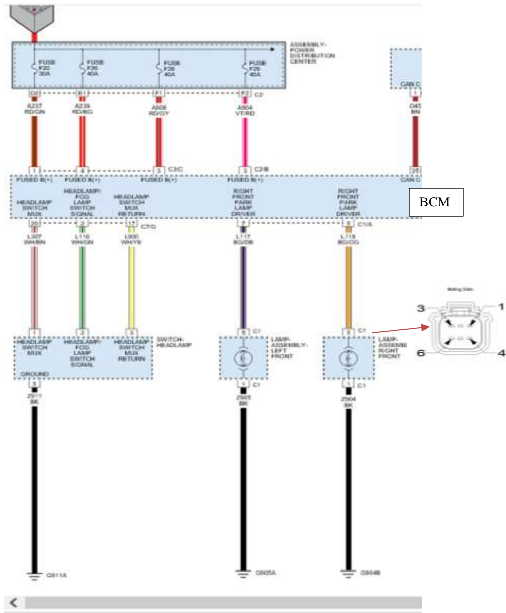
Wiring Diagram - PARK LAMPS SYSTEM
