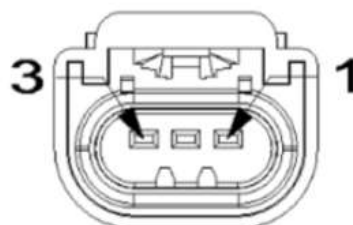
Mating Connector
