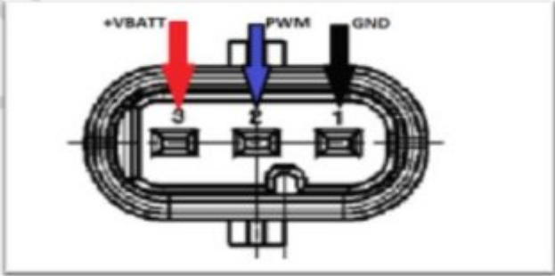
Figure 2 - Pump pin-out
