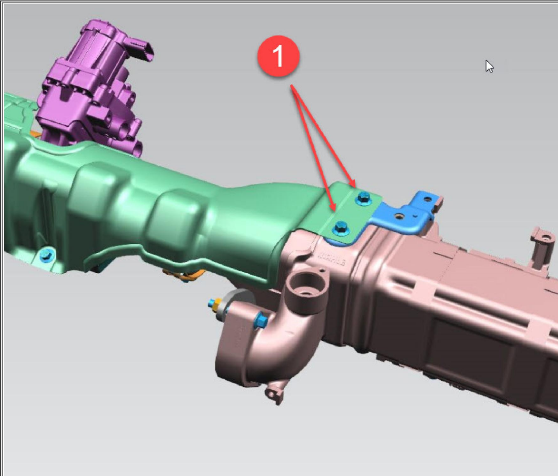
Figure #1: Former EGR Bellows Heat Shield
