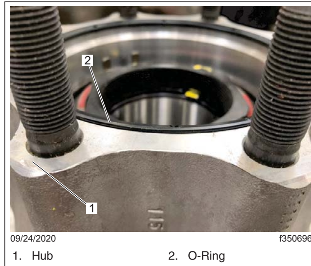
Fig. 2, O-Ring Seating
