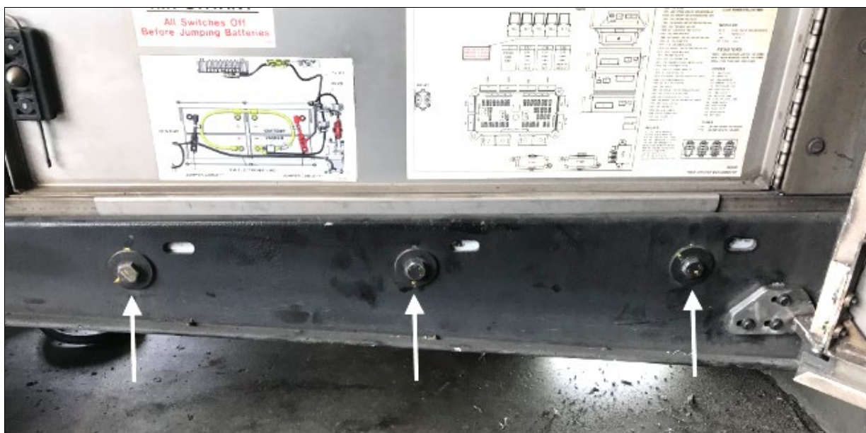
FIGURE 13: FRONT BATTERY TRAY BOLTS
