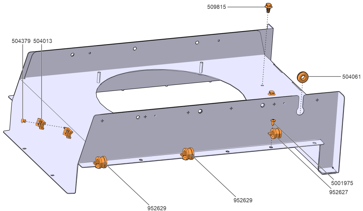
FIGURE 27: 454037 PRE-ASSEMBLY
