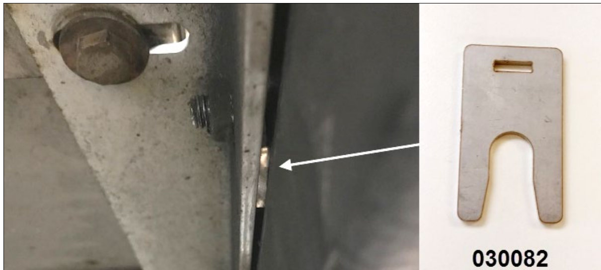
FIGURE 24 INSTALLED 030082 SHIM
