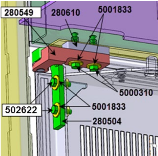
FIGURE 5: NEW UPPER HINGE
