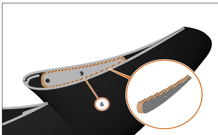
Extract from SCB 15 A 002 WI – Application area of adhesive (6)
