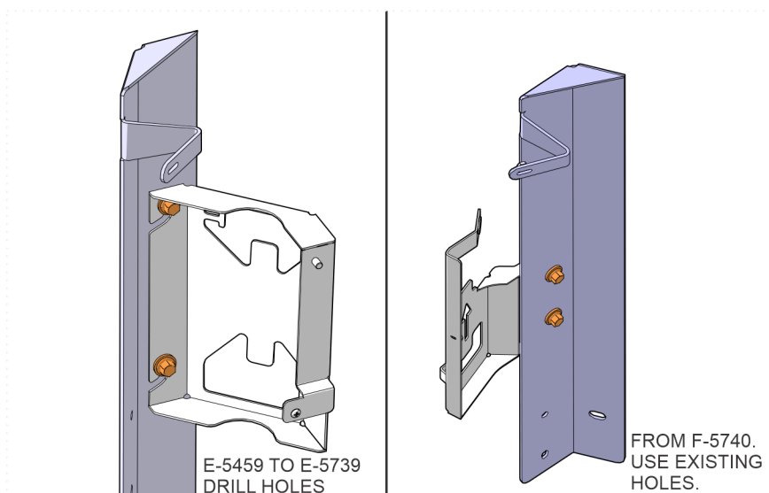
FIGURE 31: FILTER DRYER BRACKET ON POST
