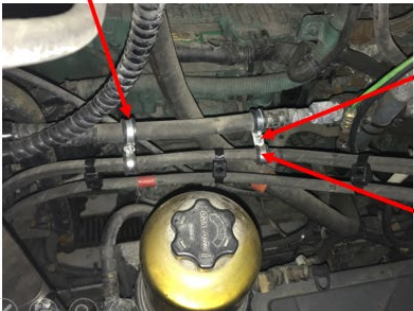
FIGURE 28: A/C HOSE ROUTING
