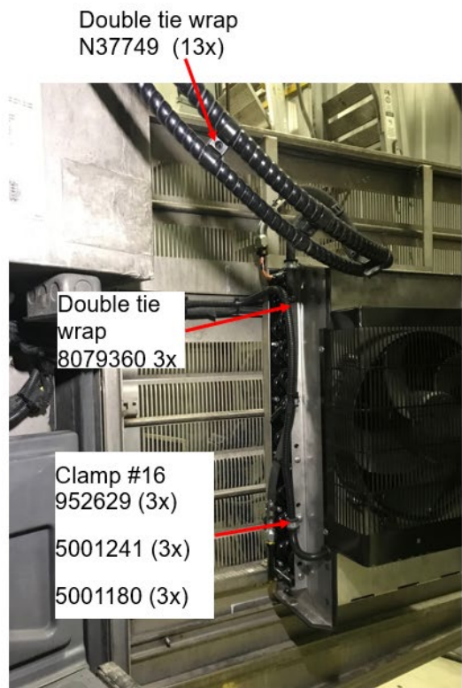
6 Internal TSD FIGURE 27: NEW CONDENSER, FAN AND ACCESSORIES
