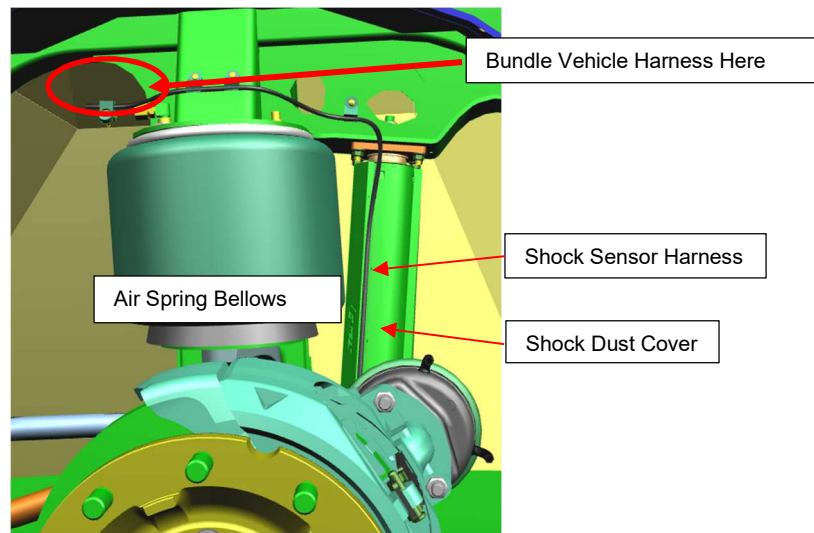
Figure 8: Curbside Shock Sensor Harness Routing.
