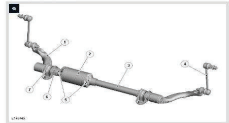
Dynamic Response Rear Actuator
