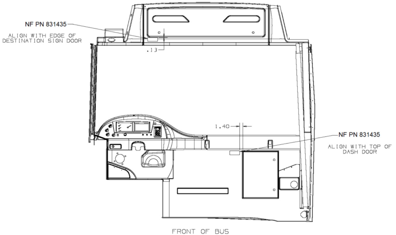
Figure 1 – Warning Label Locations
