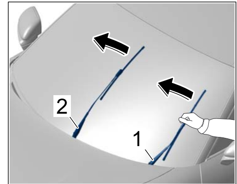
Checking wiper arm screw connections
