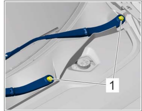
Fastening nuts for wiper arms
