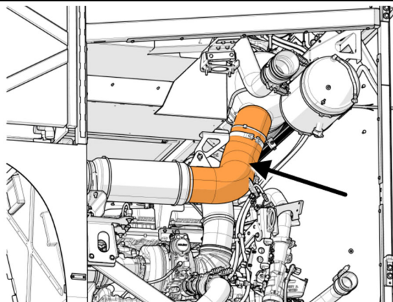
FIGURE 106: REINSTALL THIS EXHAUST PIPE SECTION
