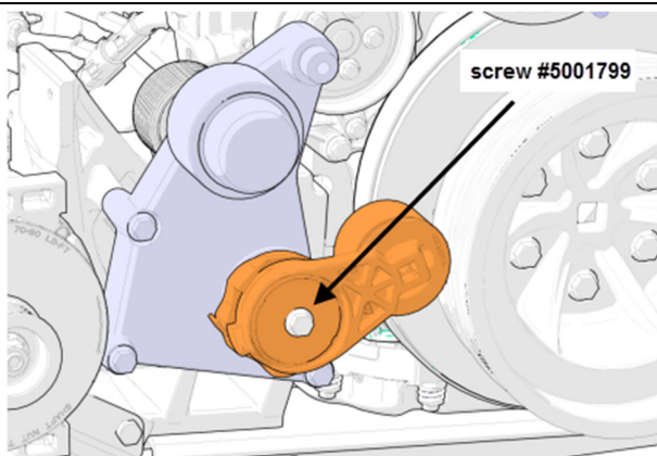
FIGURE 68: TENSIONER MOUNTING SCREW TORQUE : 48 LB-FT
