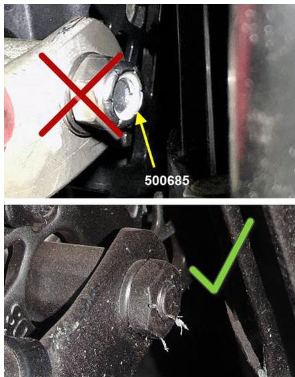
FIGURE 116: -NUT #500685 DOES NOT THREAD FULLY TO ALLOW THE LOCKING NYLON INSERT TO GRIP ON THE THREADS (UPPER IMAGE)
