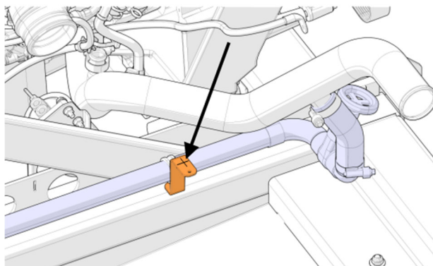
FIGURE 114: BRACKET ON THE ENGINE HOT SIDE
