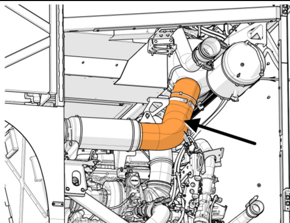
FIGURE 23: REMOVE THIS EXHAUST PIPE SECTION
