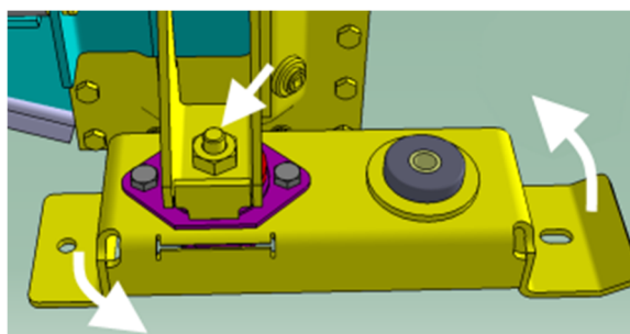
FIGURE 21: MOUNTING SUPPORT IN INITIAL POSITION
