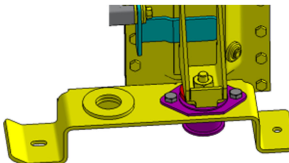
FIGURE 22: MOUNTING SUPPORT AFTER 180° ROTATION
