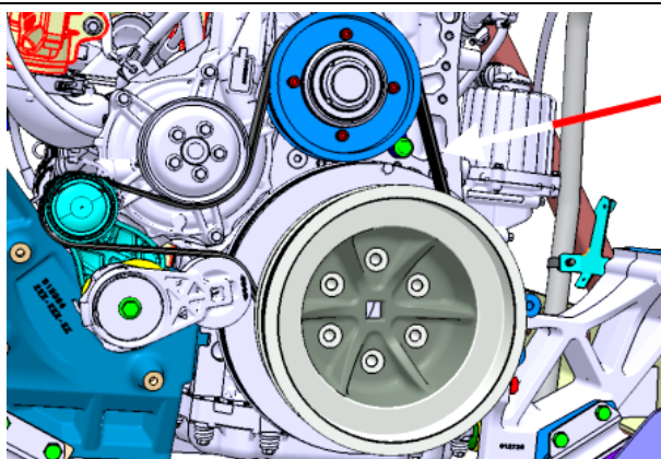
FIGURE 60: WATER PUMP DRIVE BELT
