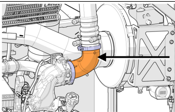
FIGURE 25: REMOVE THE INTAKE ELBOW
