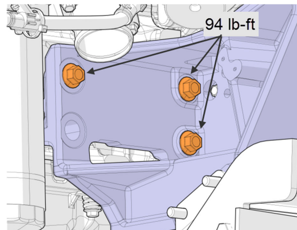
FIGURE 56: THREE (3) SCREWS ON THE SIDE OF THE ENGINE MOUNT
