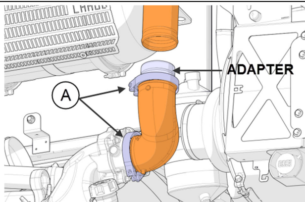
FIGURE 98: ENGINE INTAKE PIPE SUPPORT
