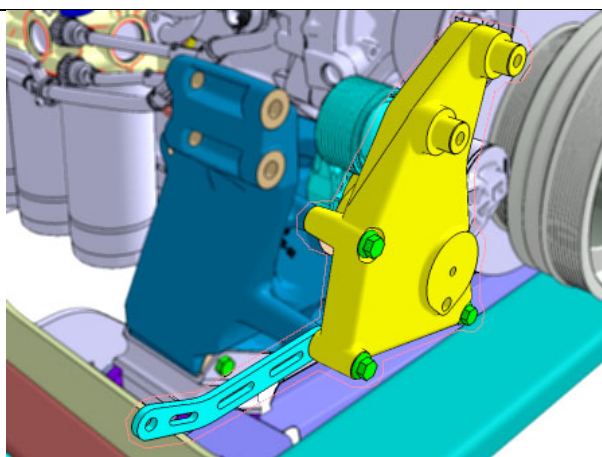
FIGURE 59: BRACKET #060102
