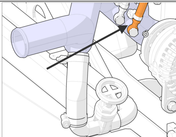
FIGURE 91: DEF INJECTOR COOLANT LINE RETURN HOSE
