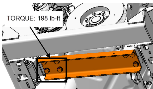
FIGURE 53: FOUR (4) SCREWS UNDER THE REINFORCEMENT CHANNEL
