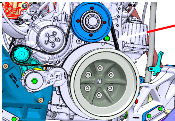
FIGURE 58: WATER PUMP DRIVE BELT
