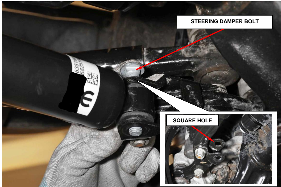
Figure 6 – Tie Rod Bracket
