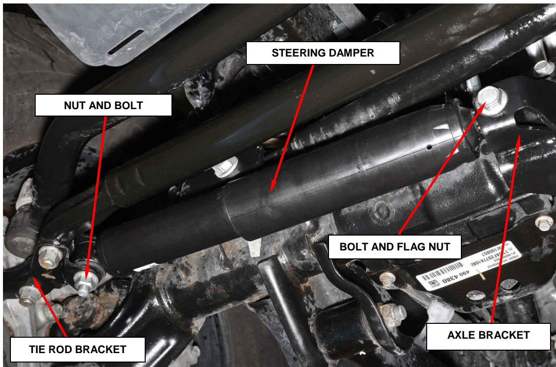
Figure 1 – Steering Damper
