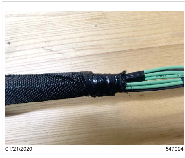
Fig. 7, Harness Wrapped with TwistTube®
