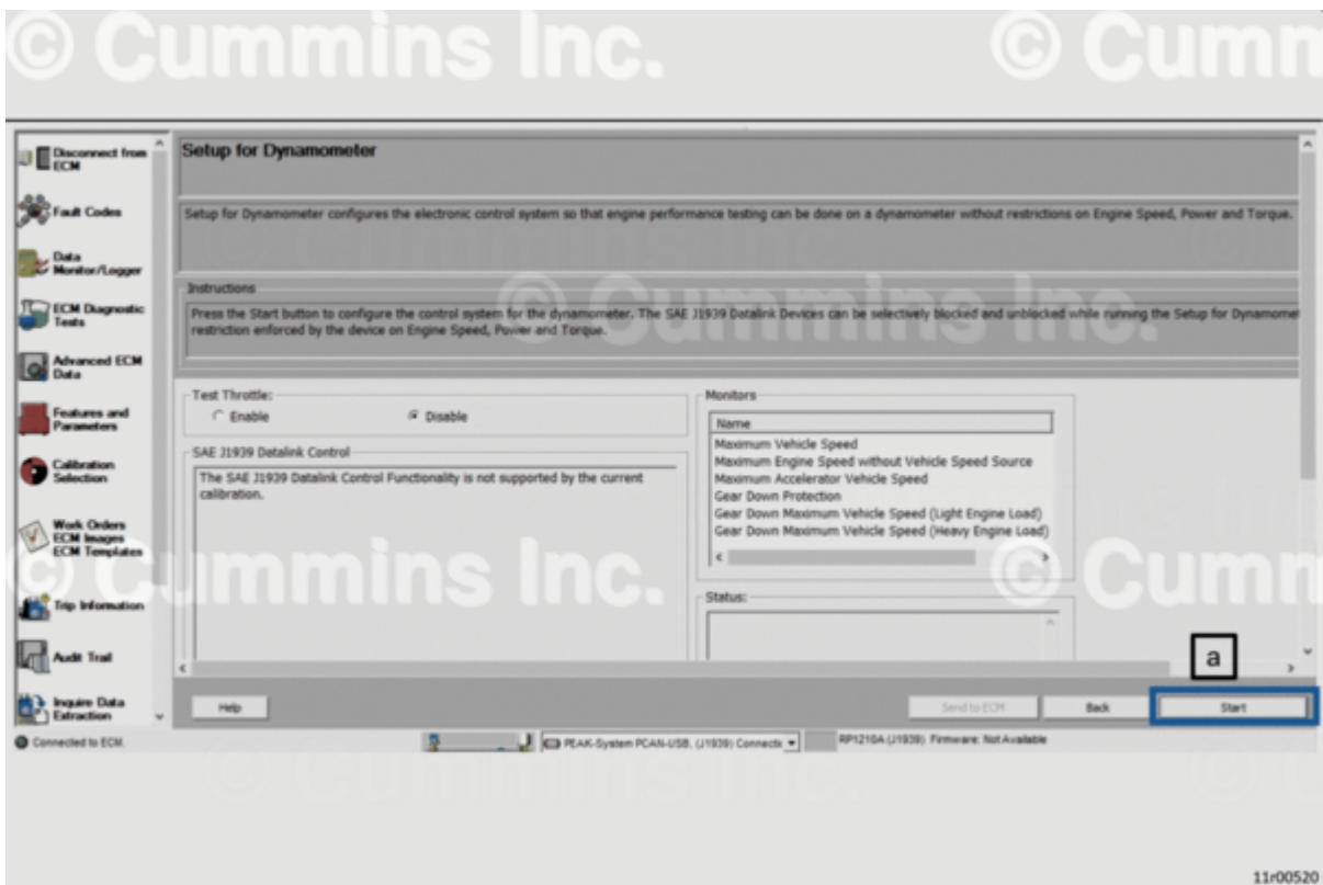
Figure 2, a. Location of “Start” Button at the Bottom of “Setup for Dynamometer” Screen.
