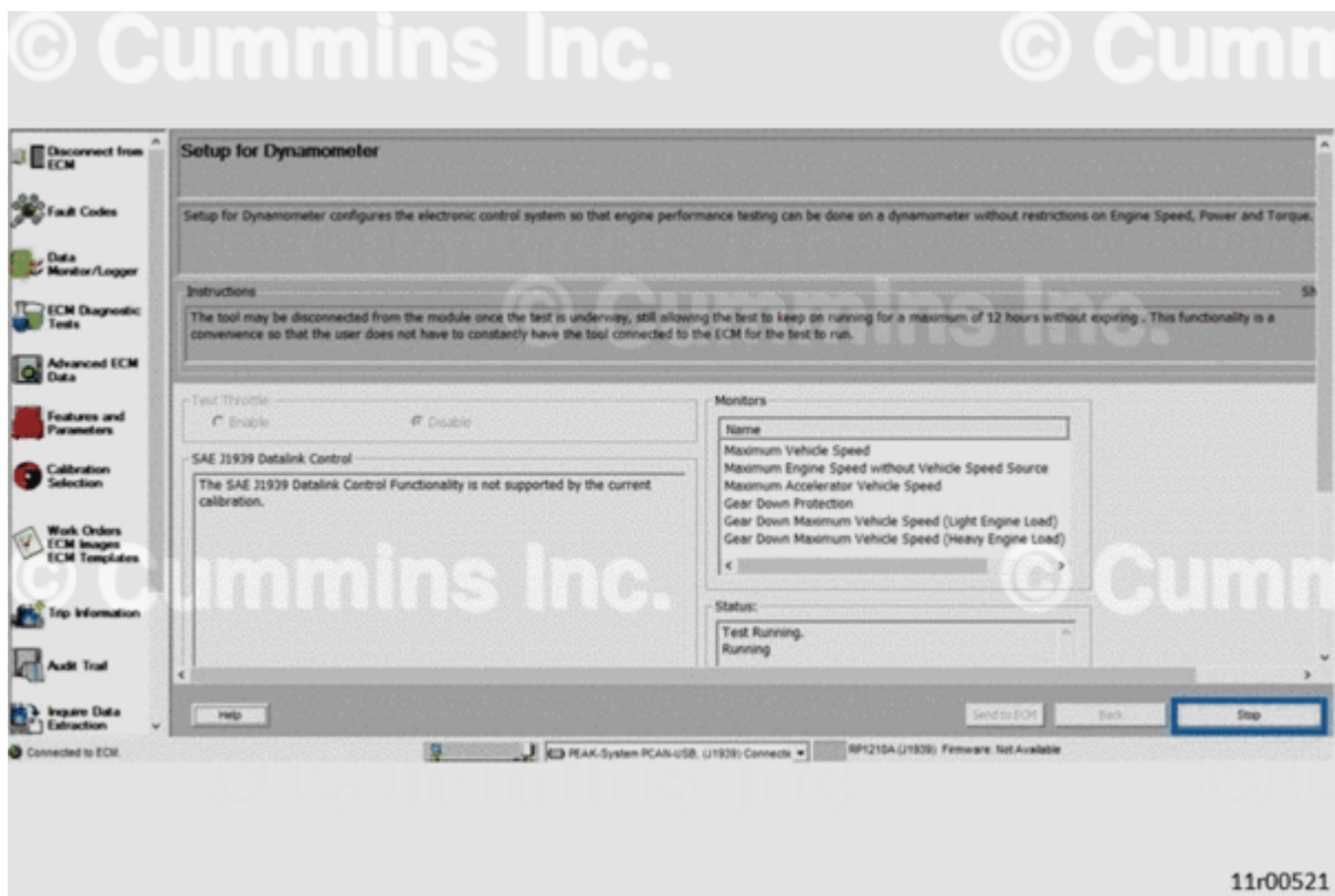
Figure 3, Location of “Stop” Button in “Setup for Dynanometer” Screen.
