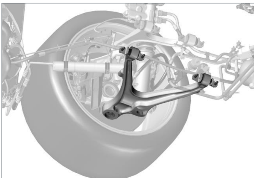
McLaren Senna Rear Lower Wishbone
