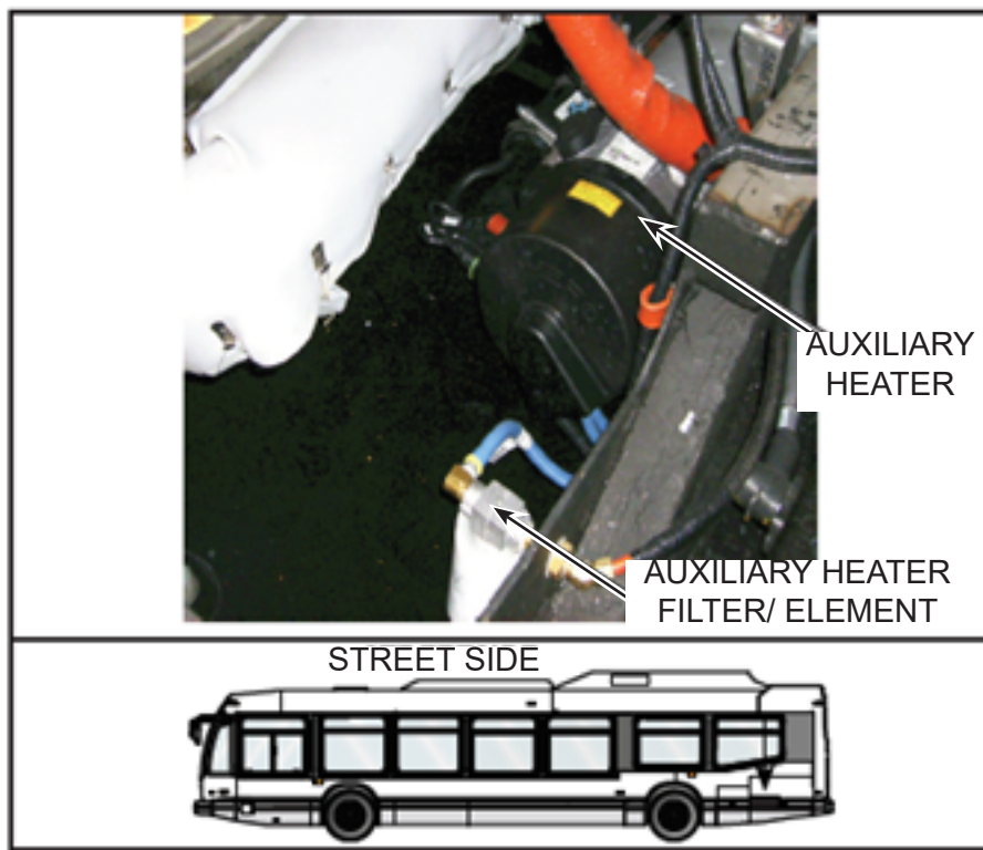
Figure 3 - View of Auxiliary Heater Fuel Filter
