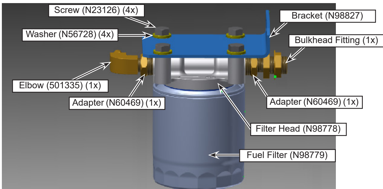
Figure 5 - Assembly of Fuel Filter, Filter Head, Fittings to the Mounting Bracket
