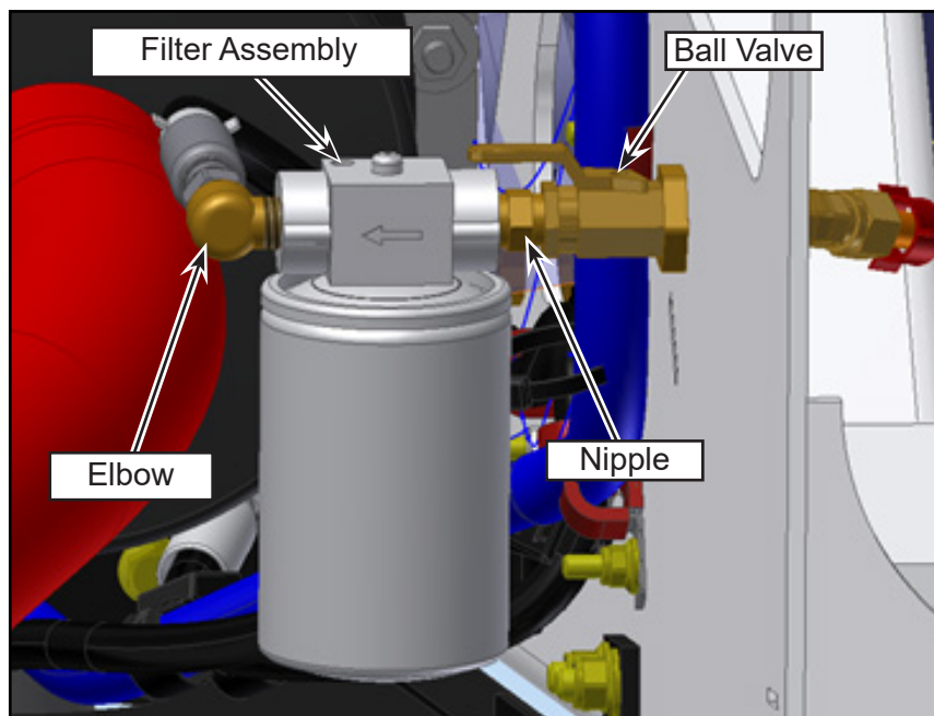
Figure 4 - Removal of Fuel Filter and Fittings
