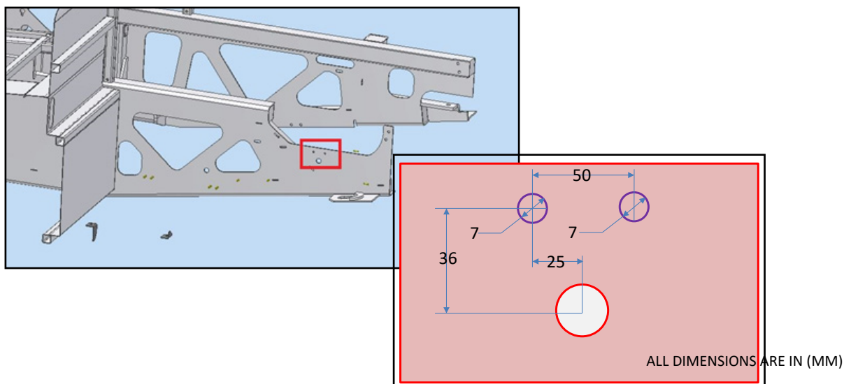
Figure 6 - Drilling Location for mounting the Fuel Filter Assembly Barcket.
