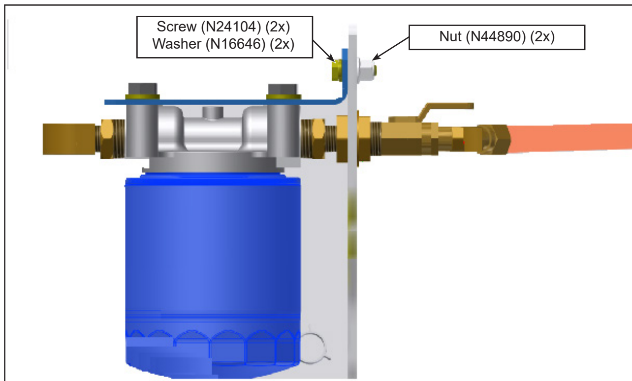
Figure 7 - Typical View of Auxiliary Heater Fuel Filter Assembly
