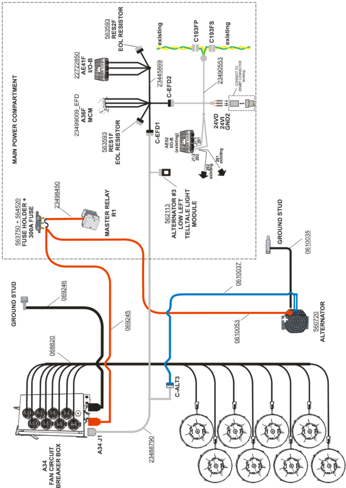
DIAGRAM OF ELECTRICAL CONNECTIONS
