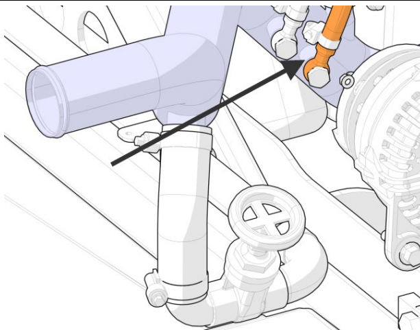
FIGURE 94: DEF INJECTOR COOLANT LINE RETURN HOSE
