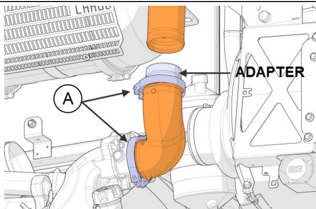
FIGURE 101: ENGINE INTAKE PIPE SUPPORT
