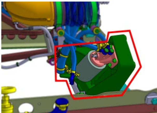
FIGURE 49: L.H. REAR ENGINE SUPPORT
