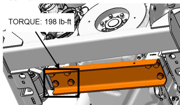
FIGURE 55: FOUR (4) SCREWS UNDER THE REINFORCEMENT CHANNEL
