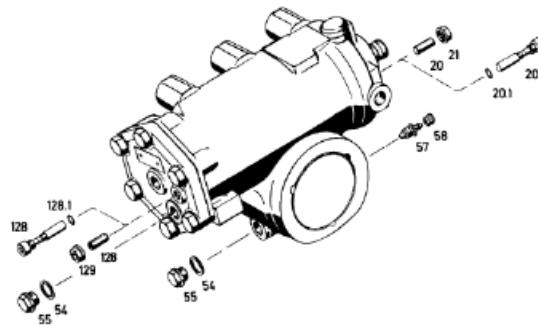
FIGURE 18 : BLEEDER (item 57) & BLEED SCREWS
