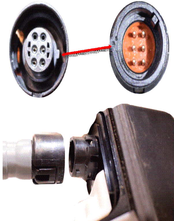
Figure 4. When installing the new reverse camera harness onto the camera assembly, ensure that the connectors are correctly aligned.
