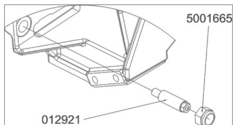
FIGURE 36: REAR VIEW – GROUND STUD
