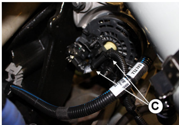
FIGURE 95: C: NYLON TIES #504016 (2x)
