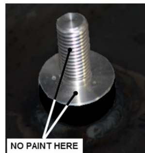
FIGURE 60: GROUND STUD #380360
