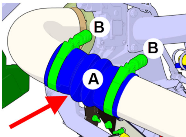
FIGURE 98: CONNECTION AT THE ENGINE INTAKE ELBOW
