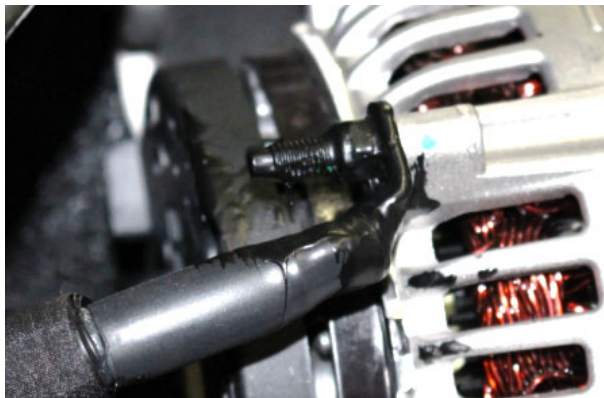
FIGURE 81: GROUND CONNECTION ON THE ALTERNATOR
