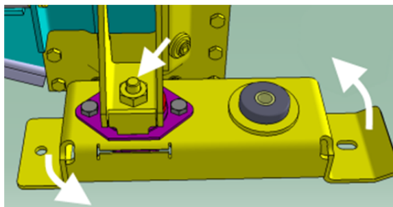
FIGURE 20: MOUNTING SUPPORT IN INITIAL POSITION
