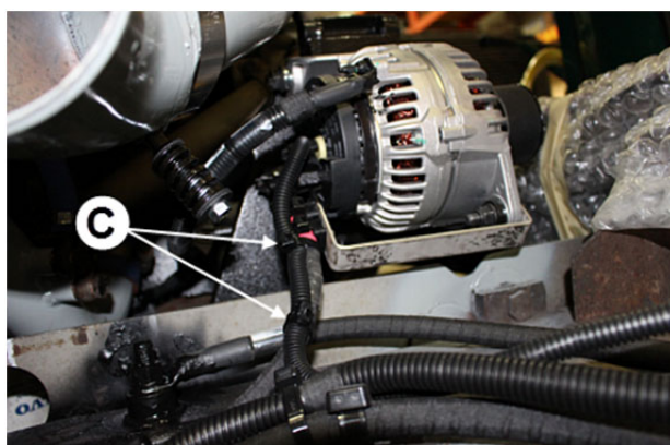
FIGURE 96: C: NYLON TIES #504016 (2x)
