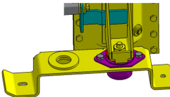
FIGURE 21: MOUNTING SUPPORT AFTER 180° ROTATION
