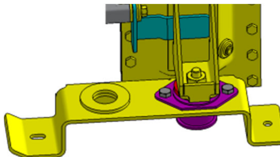
FIGURE 22: MOUNTING SUPPORT AFTER 180° ROTATION
