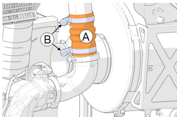
FIGURE 104: CONNECTION AT THE ENGINE INTAKE ELBOW
