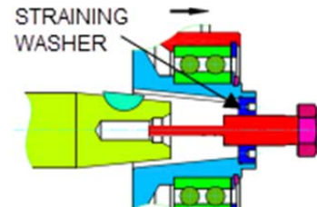
TAKE OFF THE ROTOR FIGURE 11
