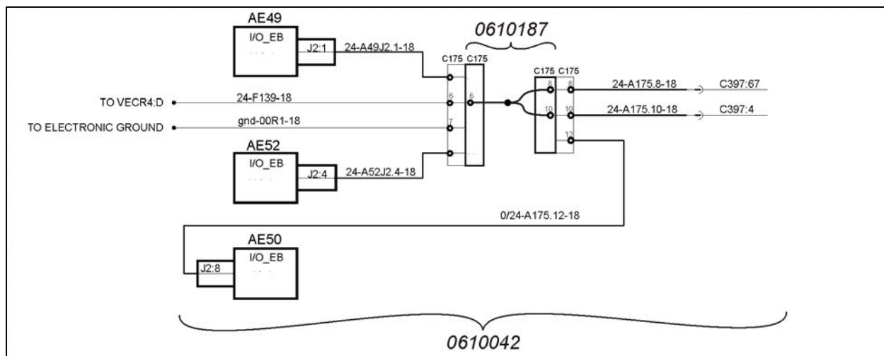
FIGURE 3: 0610042 & 0610187 HARNESS CONNECTIONS IN MAIN POWER COMPARTMENT
