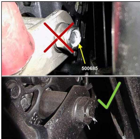
FIGURE 76: HARDWARE TO USE WITH EARLY VERSIONS
