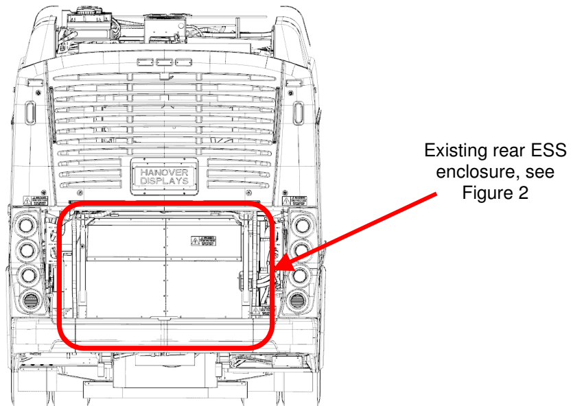
Figure 1: Rear ESS Enclosure Location (Rear Engine Door Removed for Clarity)
