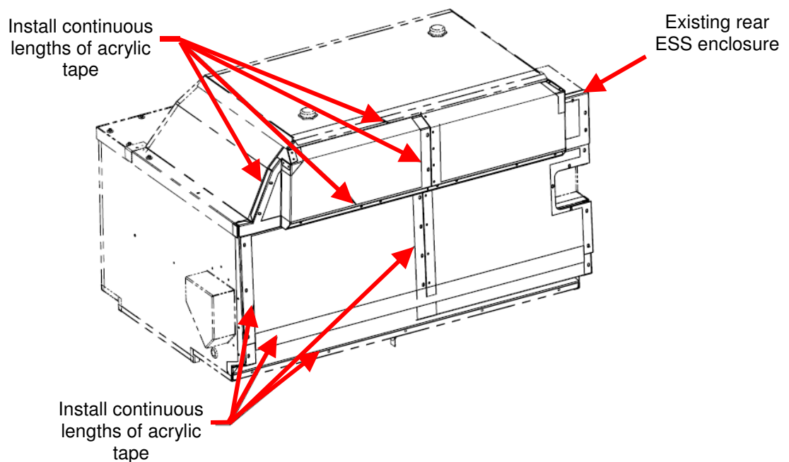
Figure 2a: Street Side Rear ESS Covers Tape Installation
